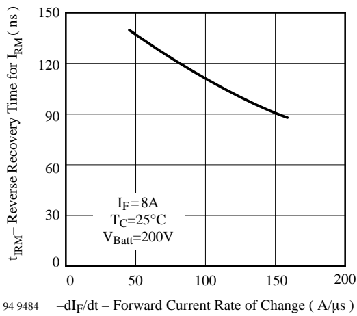
Figure 7 : Reverse Recovery Time for IRM vs. Forward Current Rate of Change
